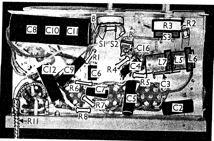
Under-chassis view. R11 is incorporated in the mains lead. C3 is a small fixed capacity. S1 and S2 are ganged in a simple rotary unit, of which two tags are blank.
